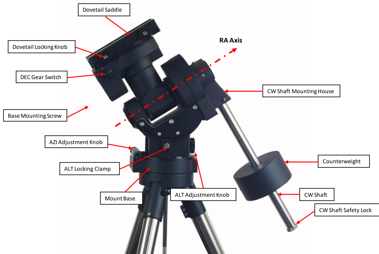
Figure 1. CEM70 mount assembly
