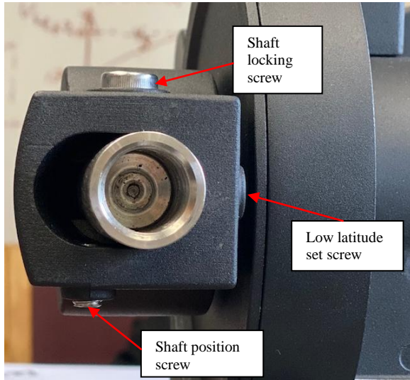
Figure 19. Screws for CW shaft tilting
