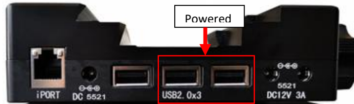
Figure 7. Ports on CEM70 dovetail saddle
