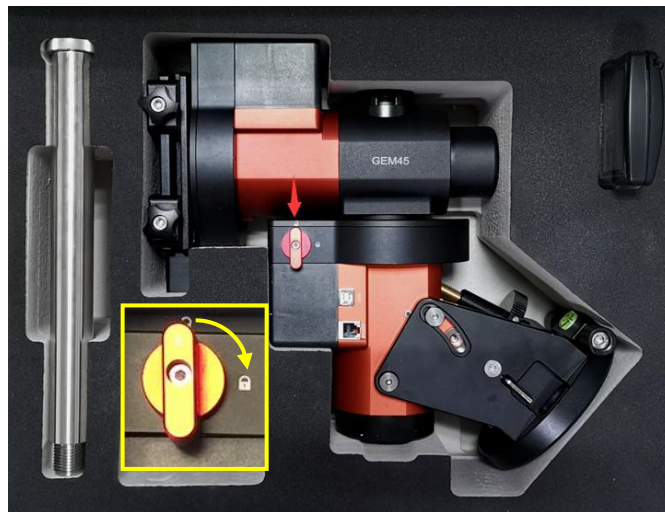
Figure 10. Mount in a hard case
