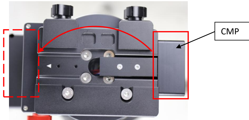
Figure 6. Top of the dovetail saddle
