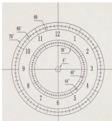
Figure 23. Polar Scope
