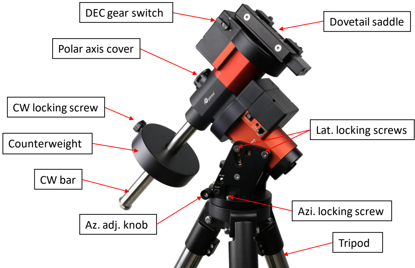
Figure 1. GEM45 mount assembly
