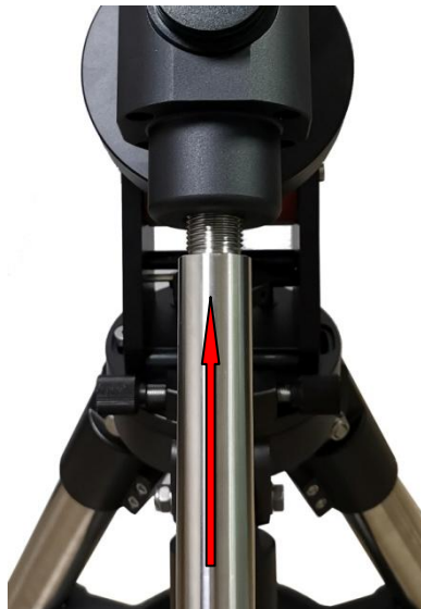
Figure 16. Install CW shaft
