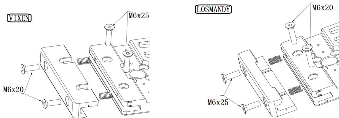
Figure 18. Switch the dovetail saddle from Vixen to Losmandy (Stationary Side)
